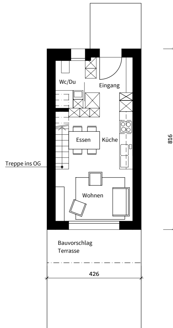
Erdgeschoss ground floor
